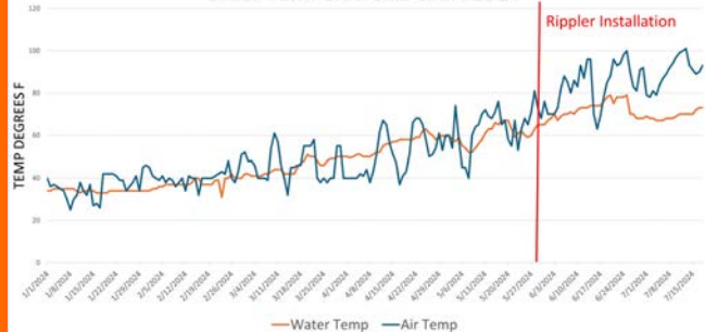
DAILY TEMPERATURE DATA 2024
